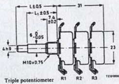
Triple potentiometer
