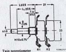
Twin potentiometer
